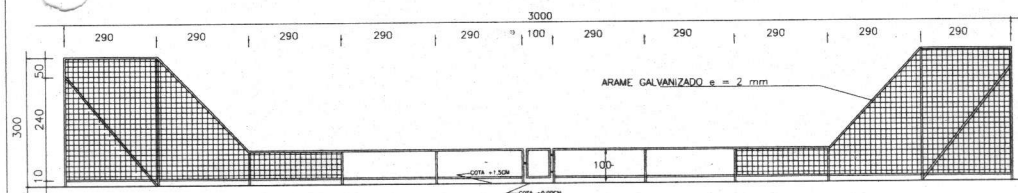
ALAMBRADO LATERAL 2 ESCALA = 1/100
