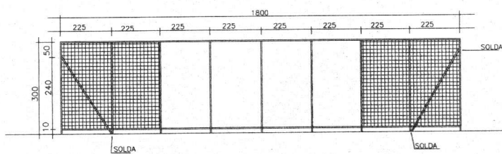
ALAMBRADO FUNDOS ESCALA = 1/100
